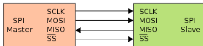
Figur 17, SPI master/slave
